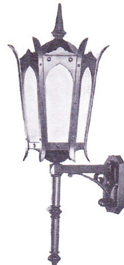
NO. C-230: Height Overall 35 1/4". Lantern size 14 1/4"x 22". Backplate 4 1/2"x 9". Wall to center 7 1/2". Maximum Watt. 300W.
