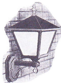
NO. 413: Height overall 18 1/2". Lantern size 9"x15". Backplate 4 1/4"x 6 3/4". Wall to center 7 1/2".
