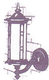
NO. 459: Height overall 19". Lantern size 6"x16". Backplate 6". Wall to center 7". Cylinder size 4"x9 5/16".
