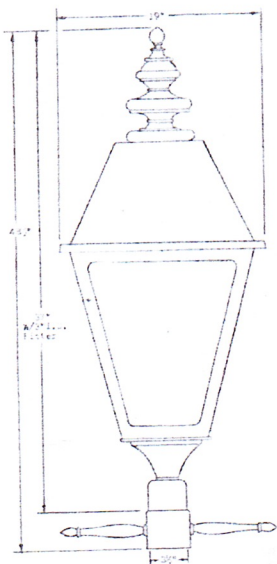
Herwig No. 2900 Lantern w/#LR-3.5 Post Fitter
