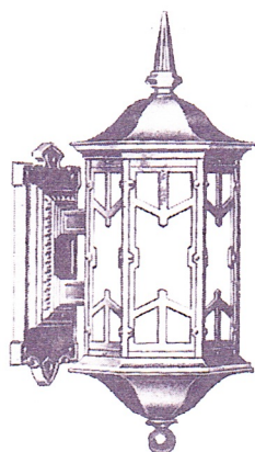
NO. D-164: Height overall 27". Lantern size 11 1/2"x27". Backplate 7 1/4"x15 1/2". Wall to center 8 1/2".
