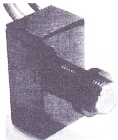
Electric Eye: Automatic Light Control for Post and Bracket Lights. Unit Totally Incased 1 1/8" x 2" x 7/8".
