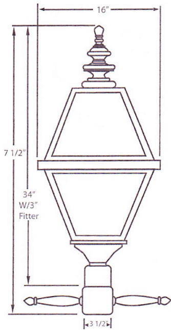
Herwig No. 3100 Lantern w/ No. LR - 3.5 Post Fitter
