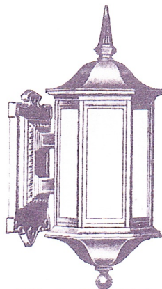
NO. P-164: Height overall 27". Lantern size 11 1/2"x27". Backplate 7 1/4"x15 1/2". Wall to center 8 1/2".
