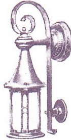
NO. S-465: Height overall 19 1/2". Lantern size 6"x12". Backplates 6" and 3 1/2". Wall to center 6 1/4". Cylinder size 4"x6".
