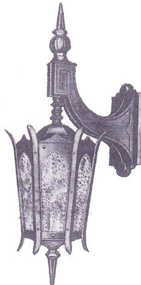
NO. A-239: Height Overall 47 1/2". Lantern size 18 1/2"x 31". Backplate 7 1/4"x 15 1/2". Wall to center 12".
