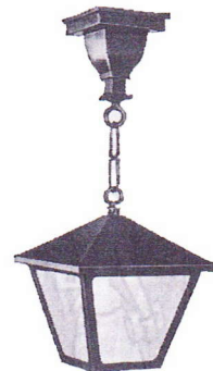
NO. 412: Height overall 36". Lantern size 9"x11". Canopy 5 1/4".
