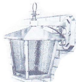
NO. 405: Height overall 18 1/2". Lantern size 11"x12 1/2" Backplate 4 1/2"x9". Wall to center 10 1/4".
