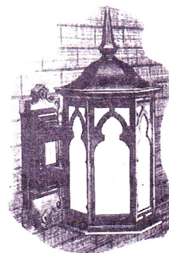
NO. G-508: Height overall 23 1/2". Lantern size 11 1/2"x22". Backplate 7 1/4"x15 1/2". Wall to center 8 1/2".
