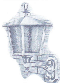
NO. 404: Height overall 27". Lantern size 11"x19 1/2" Backplate 4 1/2"x9". Wall to center 10 1/4".
