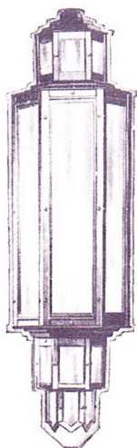
NO. 530: Height overall 34". Lantern size 9 1/4"x 33". Backplate 10 1/2"x34".
