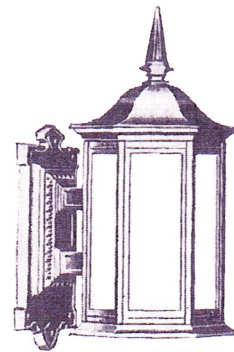
NO. P-508: Height overall 23 1/2". Lantern size 11 1/2"x22". Backplate 7 1/4"x15 1/2". Wall to center 8 1/2".
