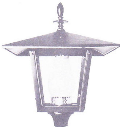
NO. 012: Height 19". Diameter at top 15". To Slip fit 3". Post C, D, E, F, or G. Maximum Watt. 150W.
