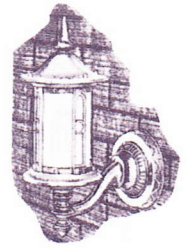
NO. 194: Height overall 15 1/2". Lantern size 6"x12 1/2". Backplate 6". Wall to center 7". Cylinder size 4"x6".
